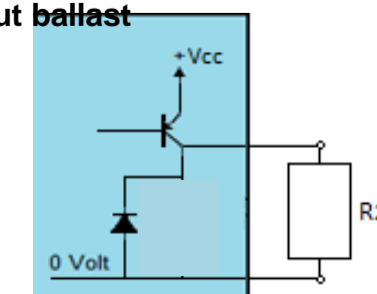
Output ballast
