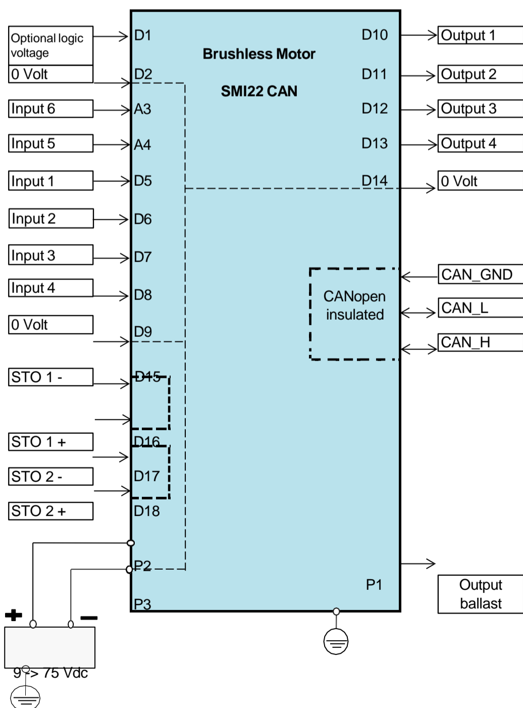
Output ballast
