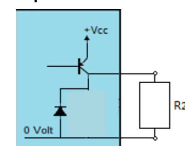
Output ballast
