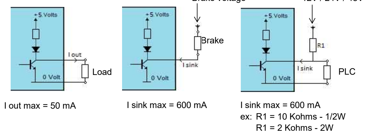
Output ballast
